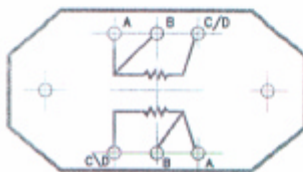
SCHEMA BORNIER SONDE A RESISTANCE TYPE DUPLEX - 2x3 FISLS
