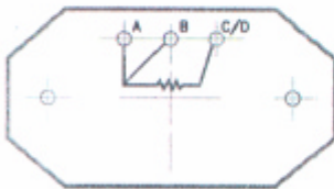
SCHEMA BORNIER SONDE A RESISTANCE TYPE SIMPLE - 3FISLS
